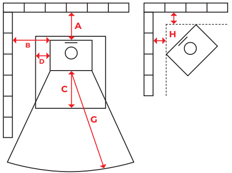
Recommended distances to non-combustibles
