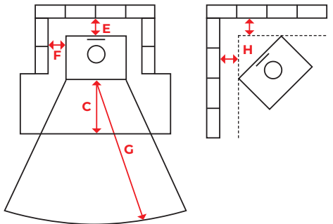
Recommended distances to non-combustibles
