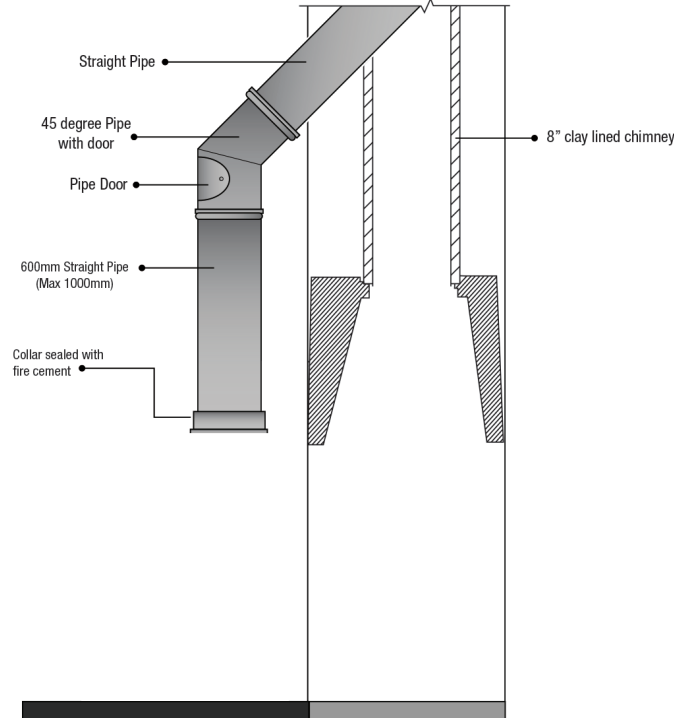
Connecting to the chimney using flue at top of the stove
