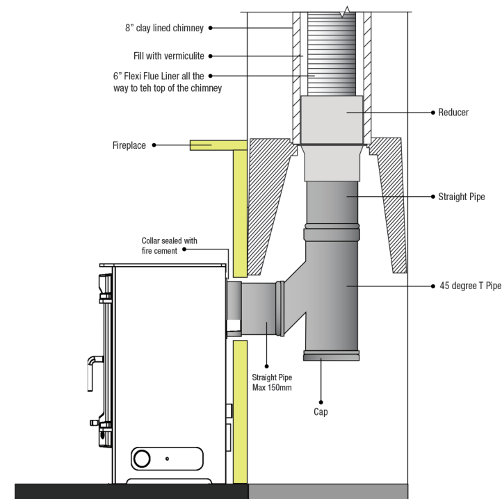
Connecting to the chimney using flue at rear of the stove
