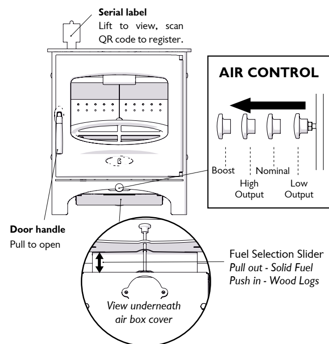
Fig. 1 Stove controls
