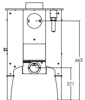
Rear
