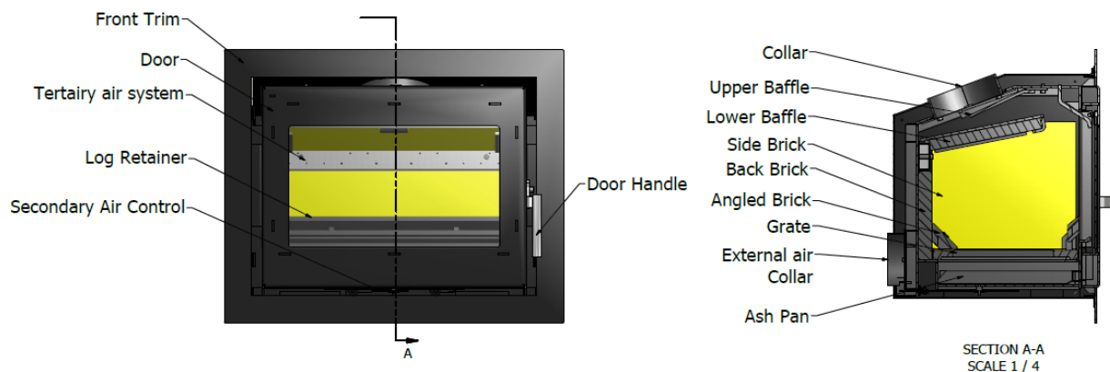
Fig 2 – Stove Assembly and controls
